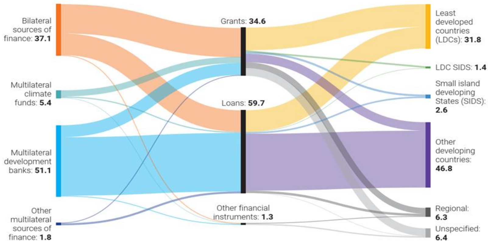
Figure 4.8 Total adaptation-specific finance commitments by finance provider type, financial instruments and LDC/SIDS status of recipient countries, 2017–2021 (US$ billions, constant prices)
